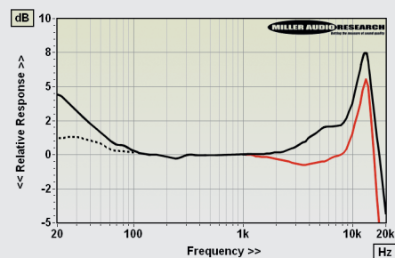
ABOVE: Frequency response curves (-8dB re. 5cm/sec) lateral (L+R, black, Output 1; dashed, Output 2) versus vertical (L-R, red Output 1)
