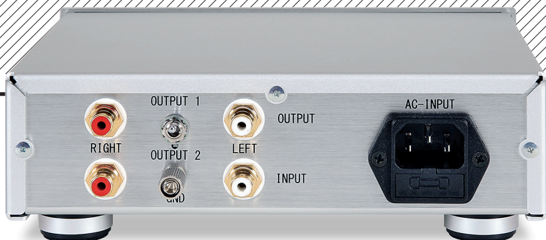
ABOVE: Rear view of the DS-E1 PSU/equaliser. The pick-up's internal LED is powered via the R- and L- pins while the output is returned via R+ and L+, all via the 'Input' RCAs. The equalised outs are also on RCAs (Output 2 with a deeper subsonic filter)
